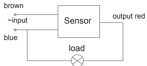
Connection-line diagram
