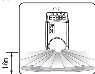
Height of installation 1-6m
