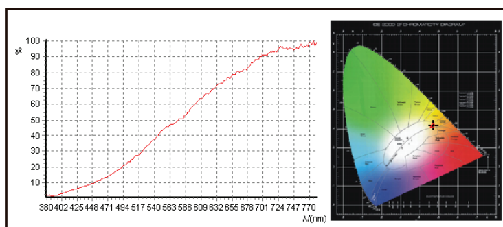
60 watt incandescent lamp(≈400lm)
