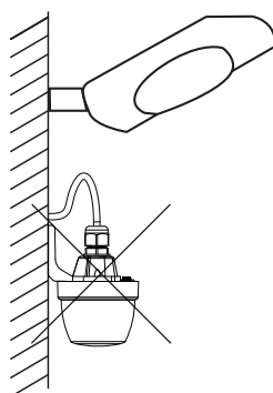
Wrong installation
